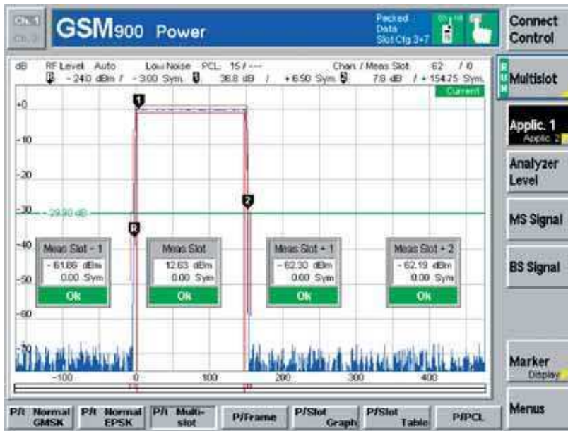
The power-versus-time multislot application can graphically display up to 4 adjacent timeslots, automatically detects GMSK- and 8PSK-modulated signals and activates the associated templates in real-time. A new zoom function allows full-screen display of each slot.
