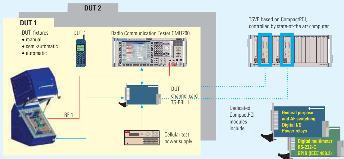
Block diagram for a 2-channel configuration of TS7100
